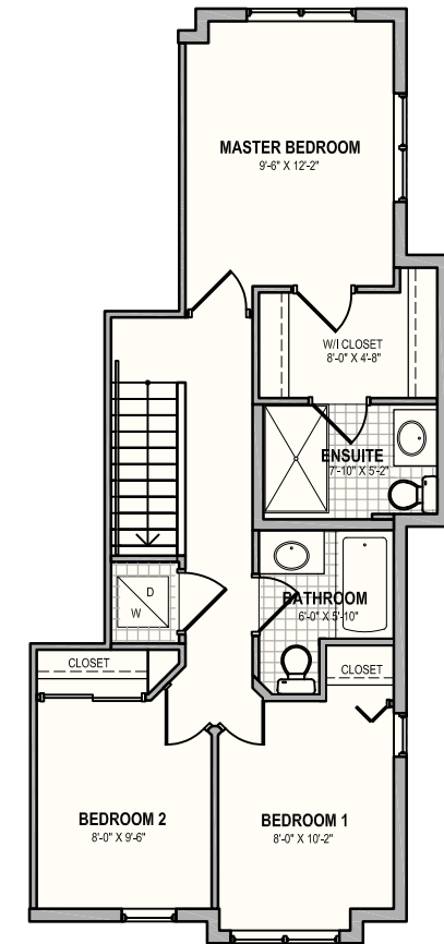
UPPER FLOOR 612 sq ft.
