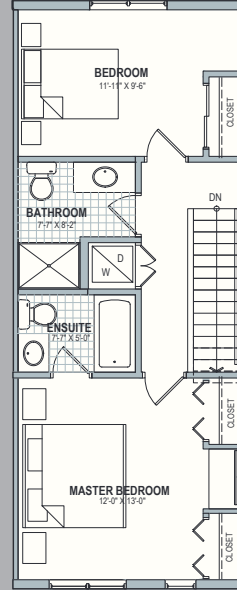
UPPER FLOOR 593 sq ft.
